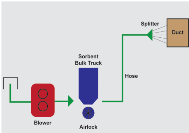
CBEEC Sorbent Injection Schematic
